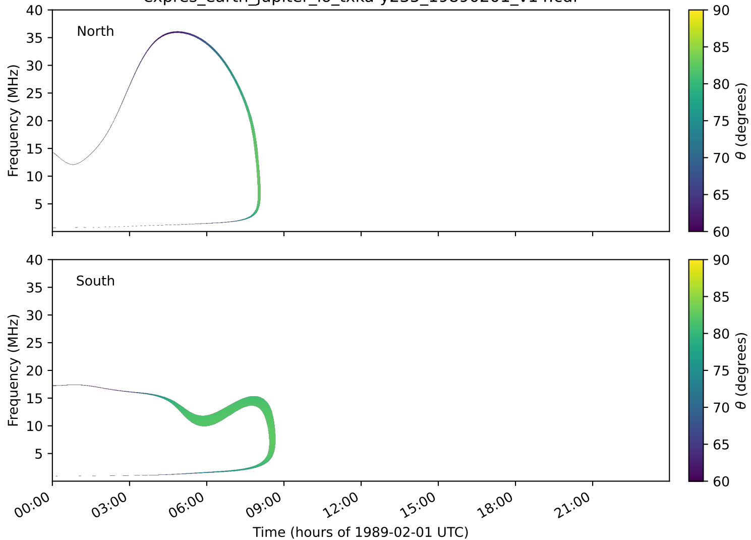
expres_earth_jupiter_io_txka-y235_19890201_v14.cdf
