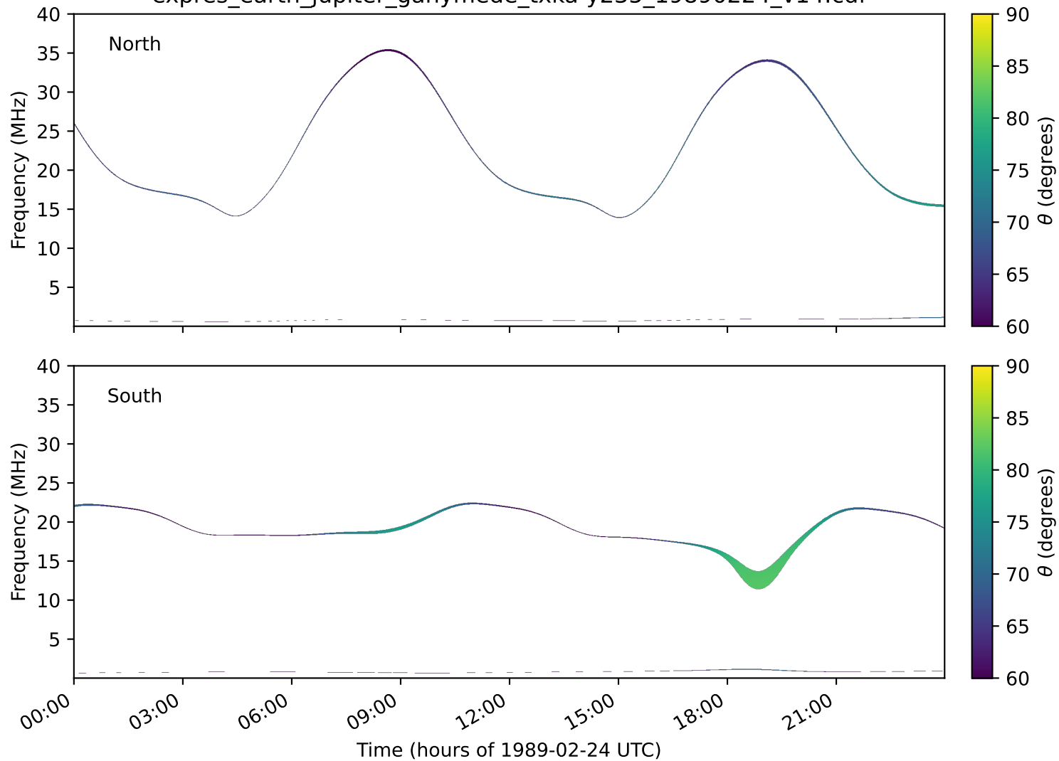
expres_earth_jupiter_ganymede_txka-y235_19890224_v14.cdf
