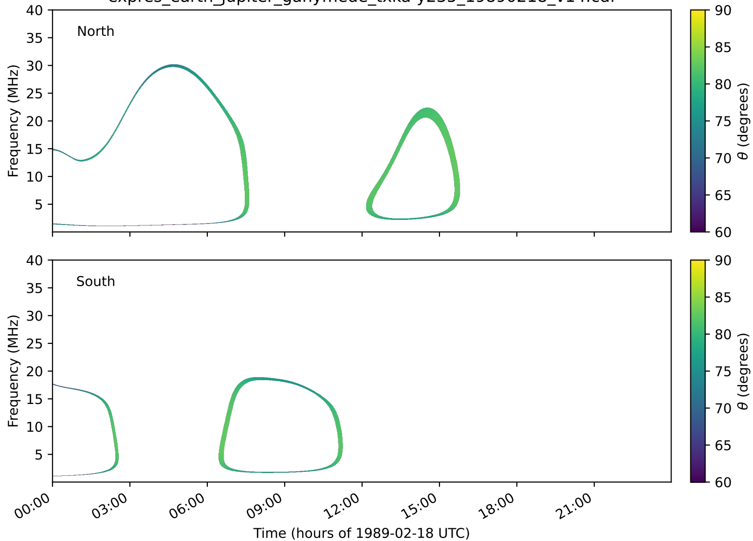
expres_earth_jupiter_ganymede_txka-y235_19890218_v14.cdf
