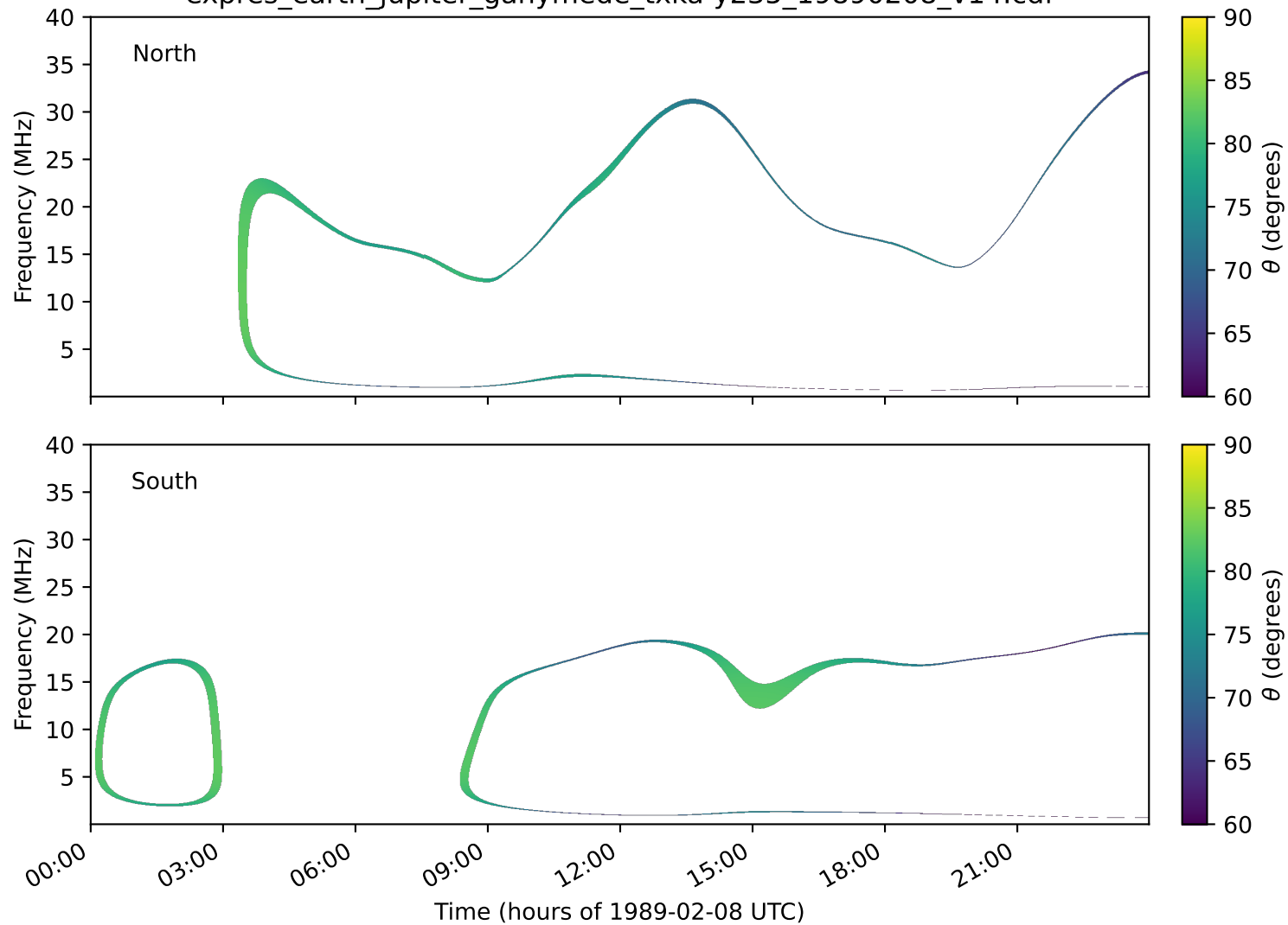
expres_earth_jupiter_ganymede_txka-y235_19890208_v14.cdf
