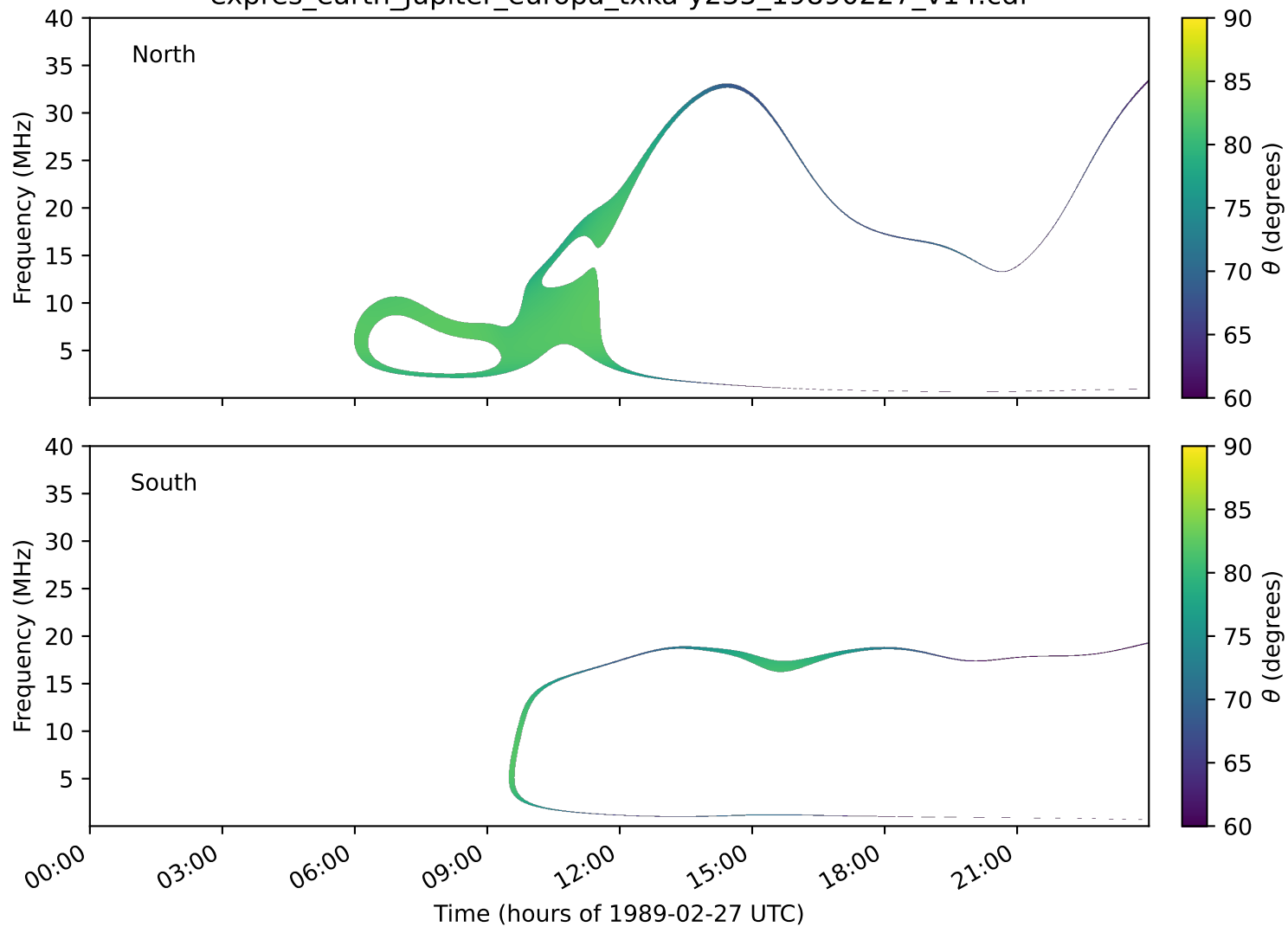
expres_earth_jupiter_europa_txka-y235_19890227_v14.cdf
