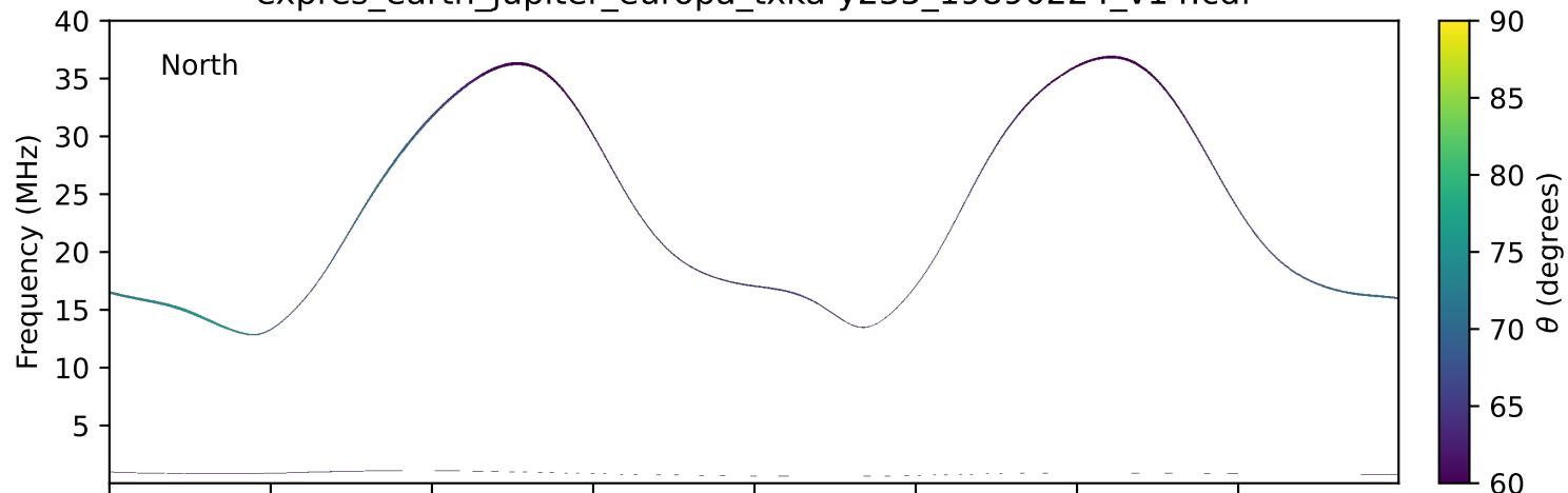
expres_earth_jupiter_europa_txka-y235_19890224_v14.cdf
