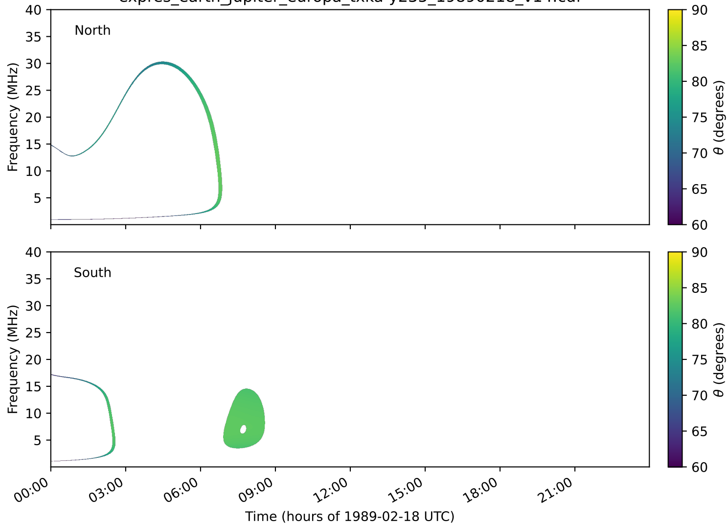
expres_earth_jupiter_europa_txka-y235_19890218_v14.cdf
