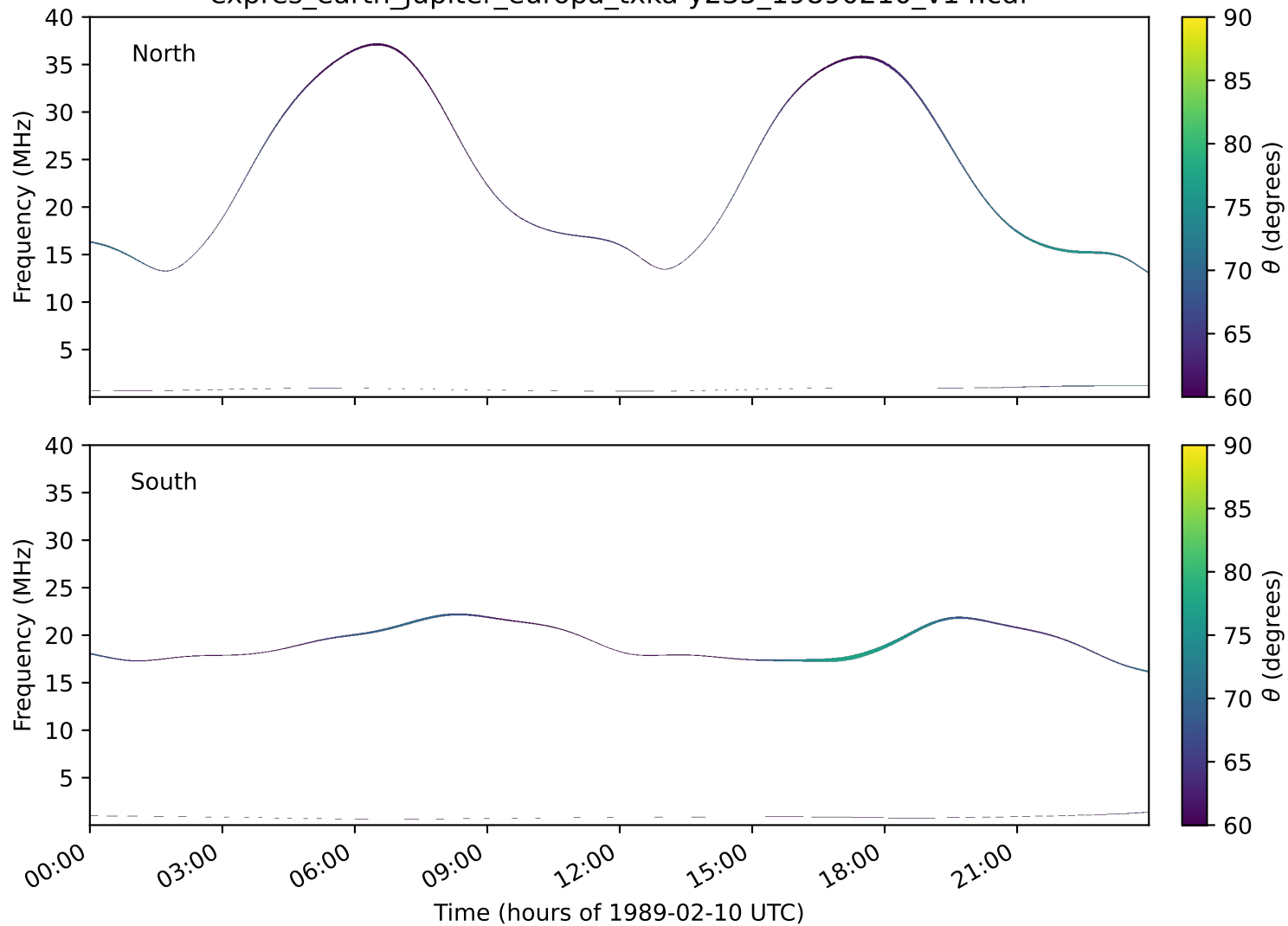
expres_earth_jupiter_europa_txka-y235_19890210_v14.cdf
