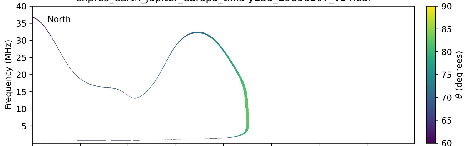
expres_earth_jupiter_europa_txka-y235_19890207_v14.cdf
