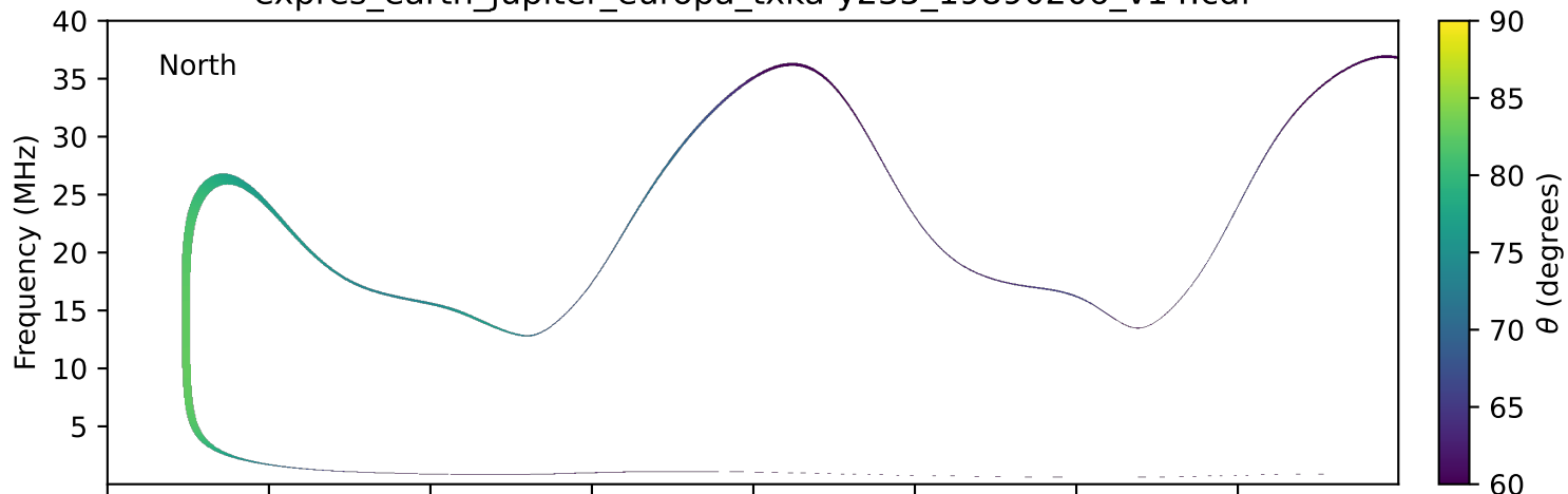
expres_earth_jupiter_europa_txka-y235_19890206_v14.cdf
