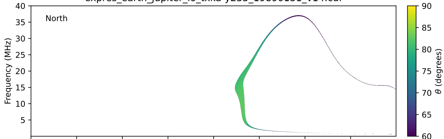
expres_earth_jupiter_io_txka-y235_19890131_v14.cdf
