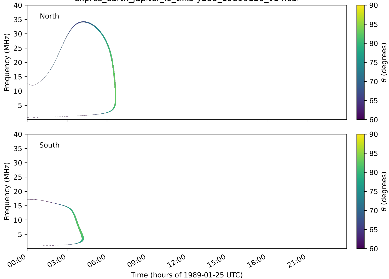
expres_earth_jupiter_io_txka-y235_19890125_v14.cdf
