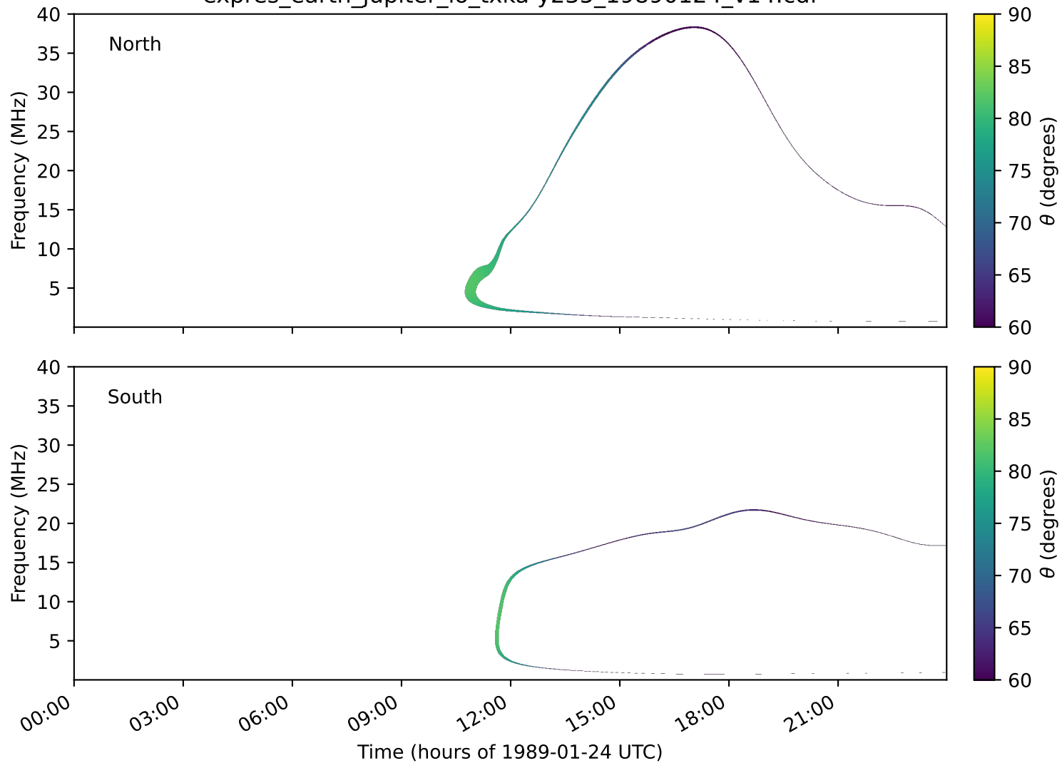
expres_earth_jupiter_io_txka-y235_19890124_v14.cdf
