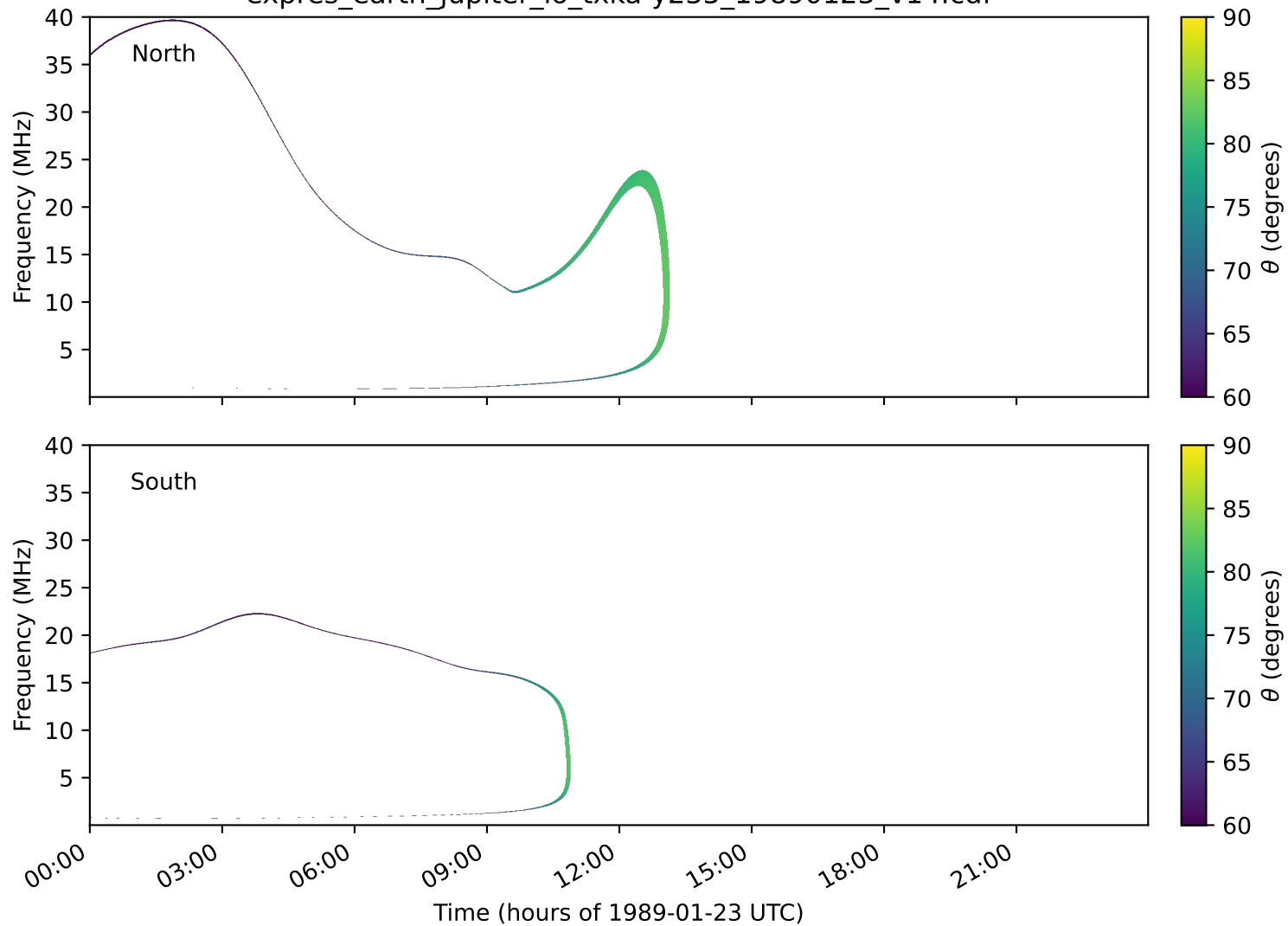
expres_earth_jupiter_io_txka-y235_19890123_v14.cdf
