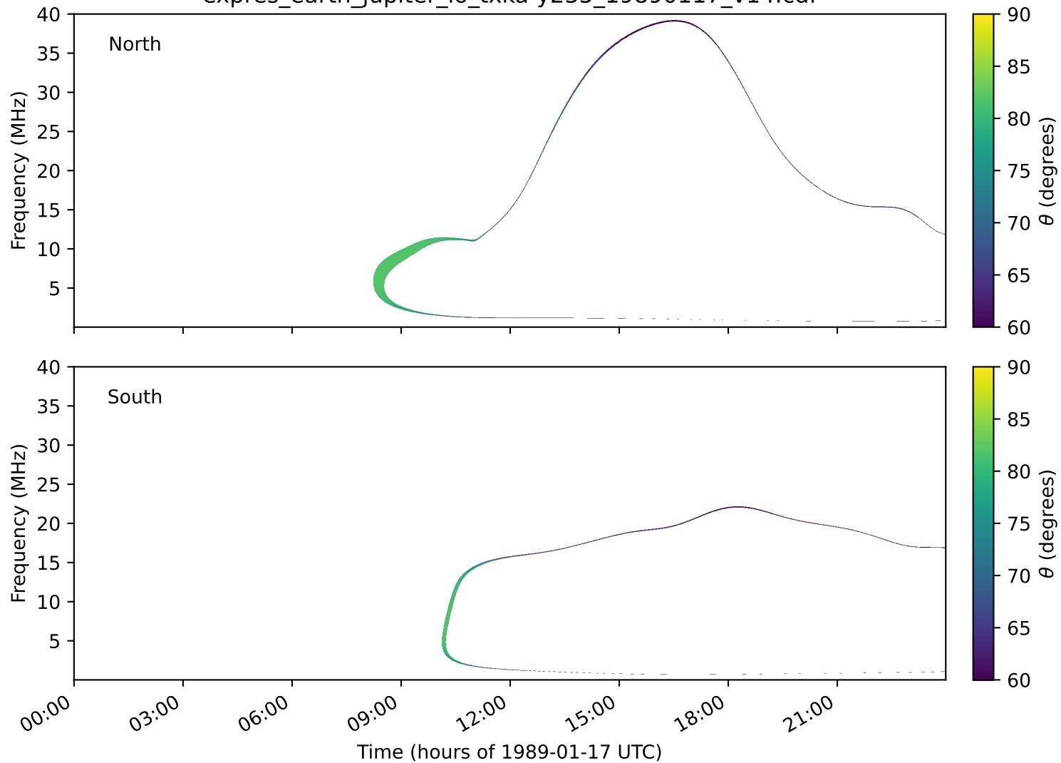
expres_earth_jupiter_io_txka-y235_19890117_v14.cdf
