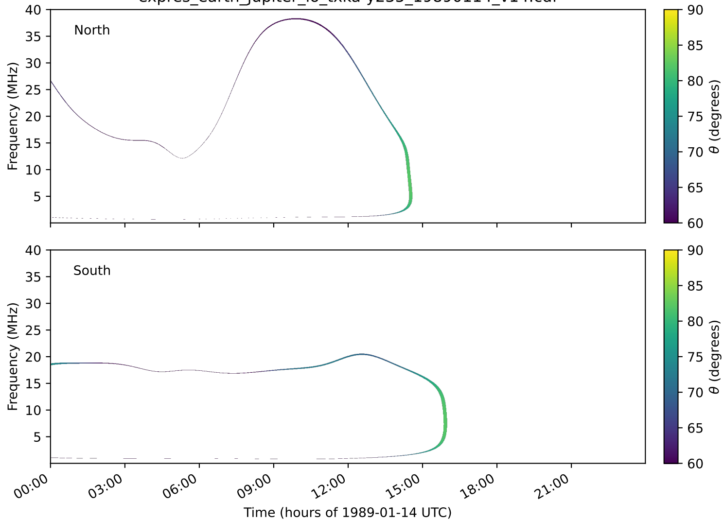
expres_earth_jupiter_io_txka-y235_19890114_v14.cdf
