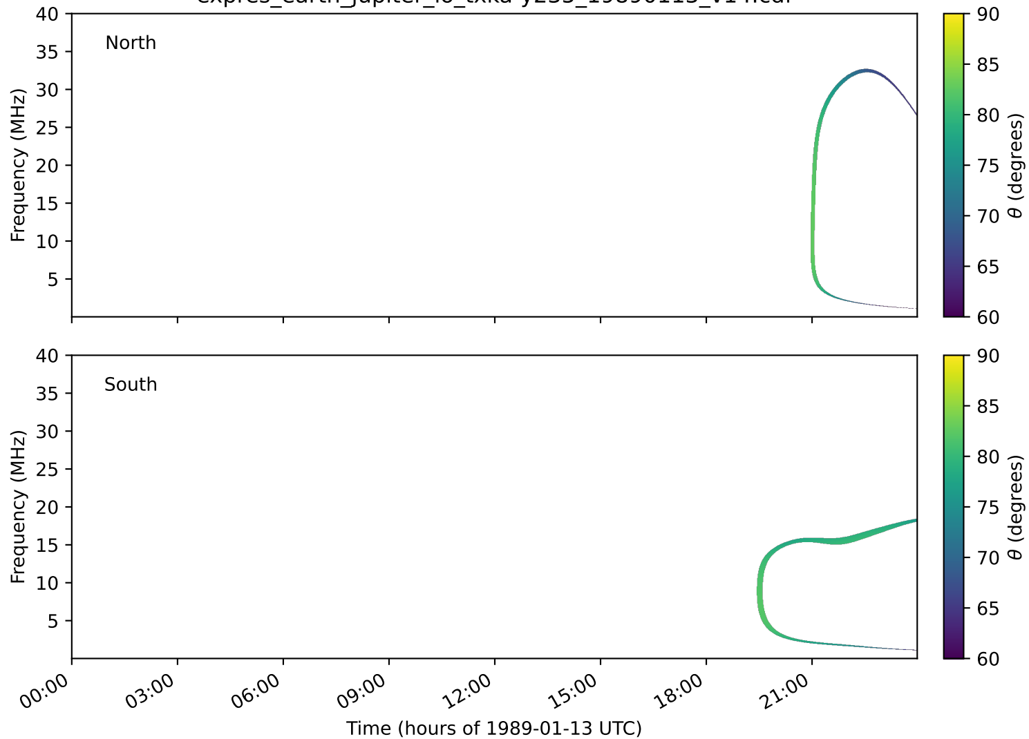
expres_earth_jupiter_io_txka-y235_19890113_v14.cdf
