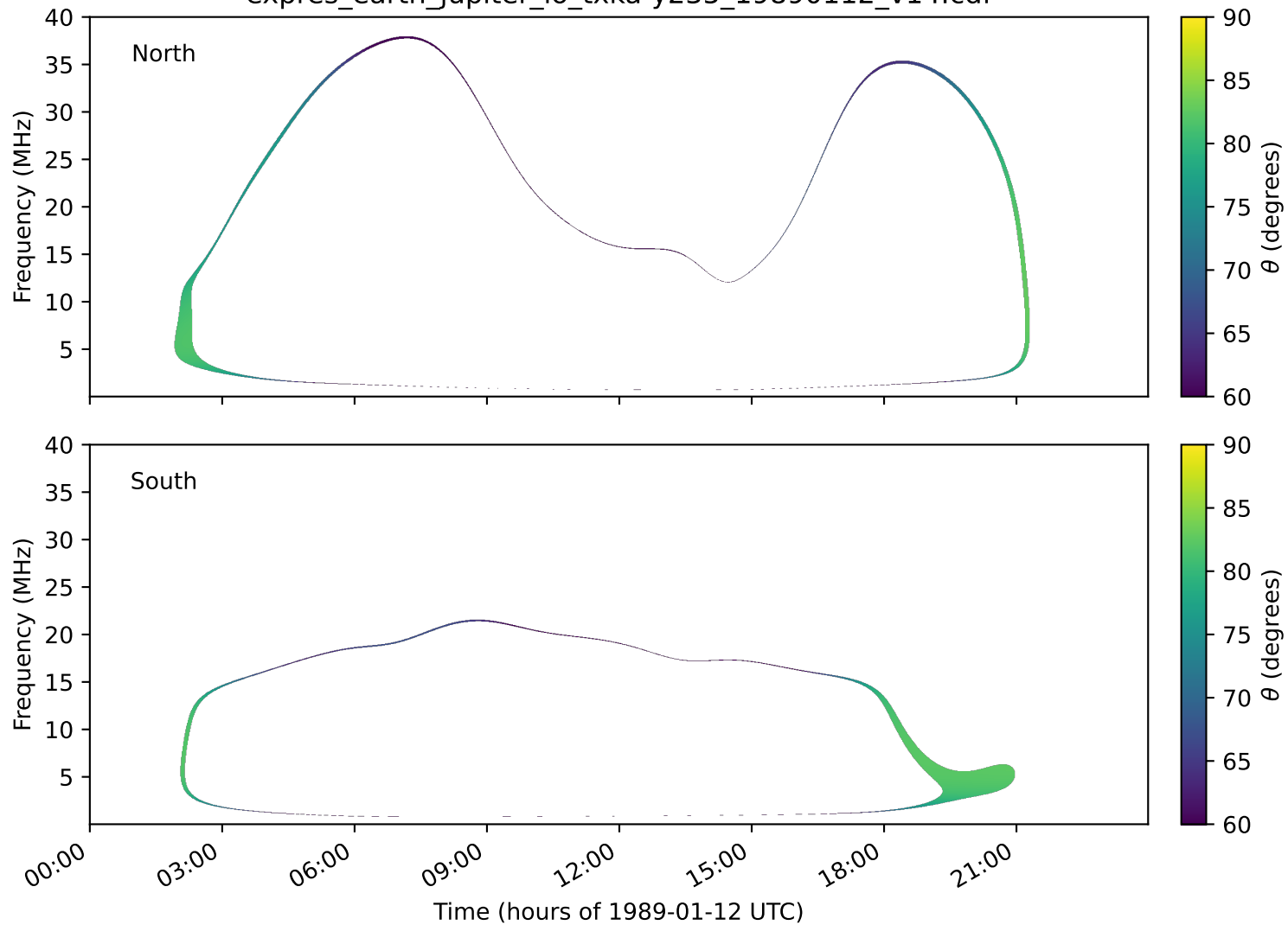
expres_earth_jupiter_io_txka-y235_19890112_v14.cdf
