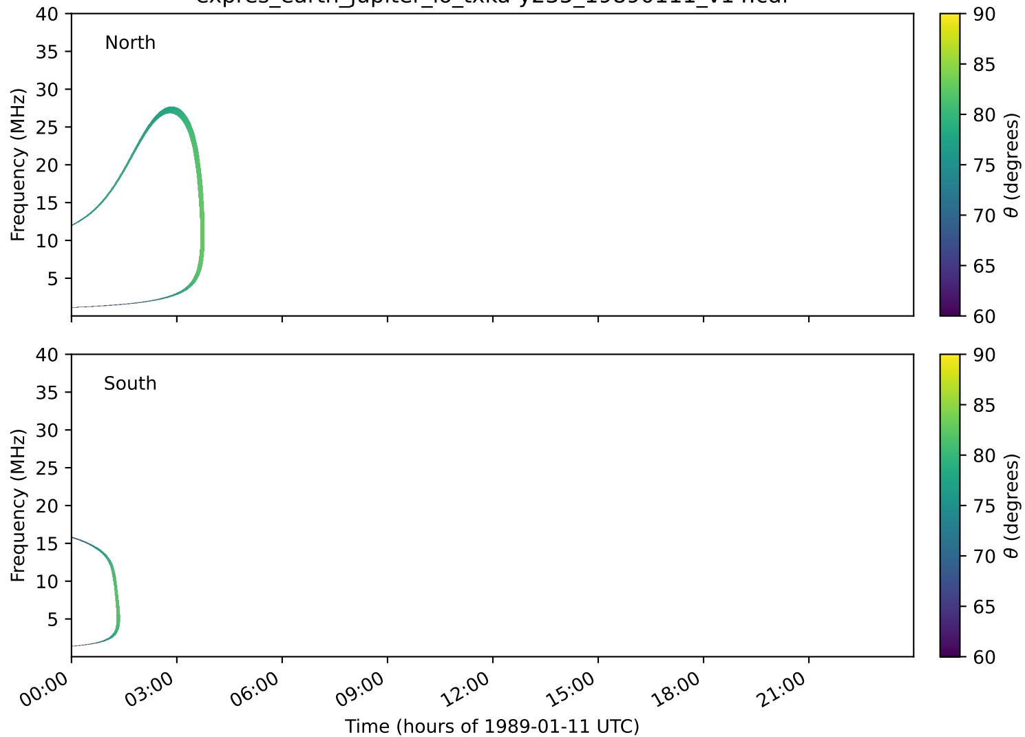
expres_earth_jupiter_io_txka-y235_19890111_v14.cdf
