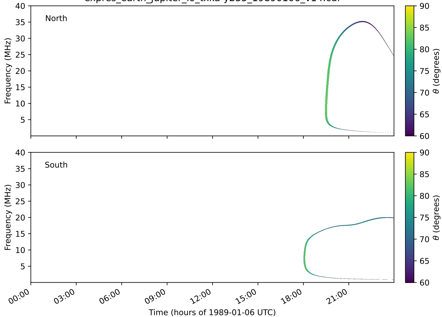
expres_earth_jupiter_io_txka-y235_19890106_v14.cdf
