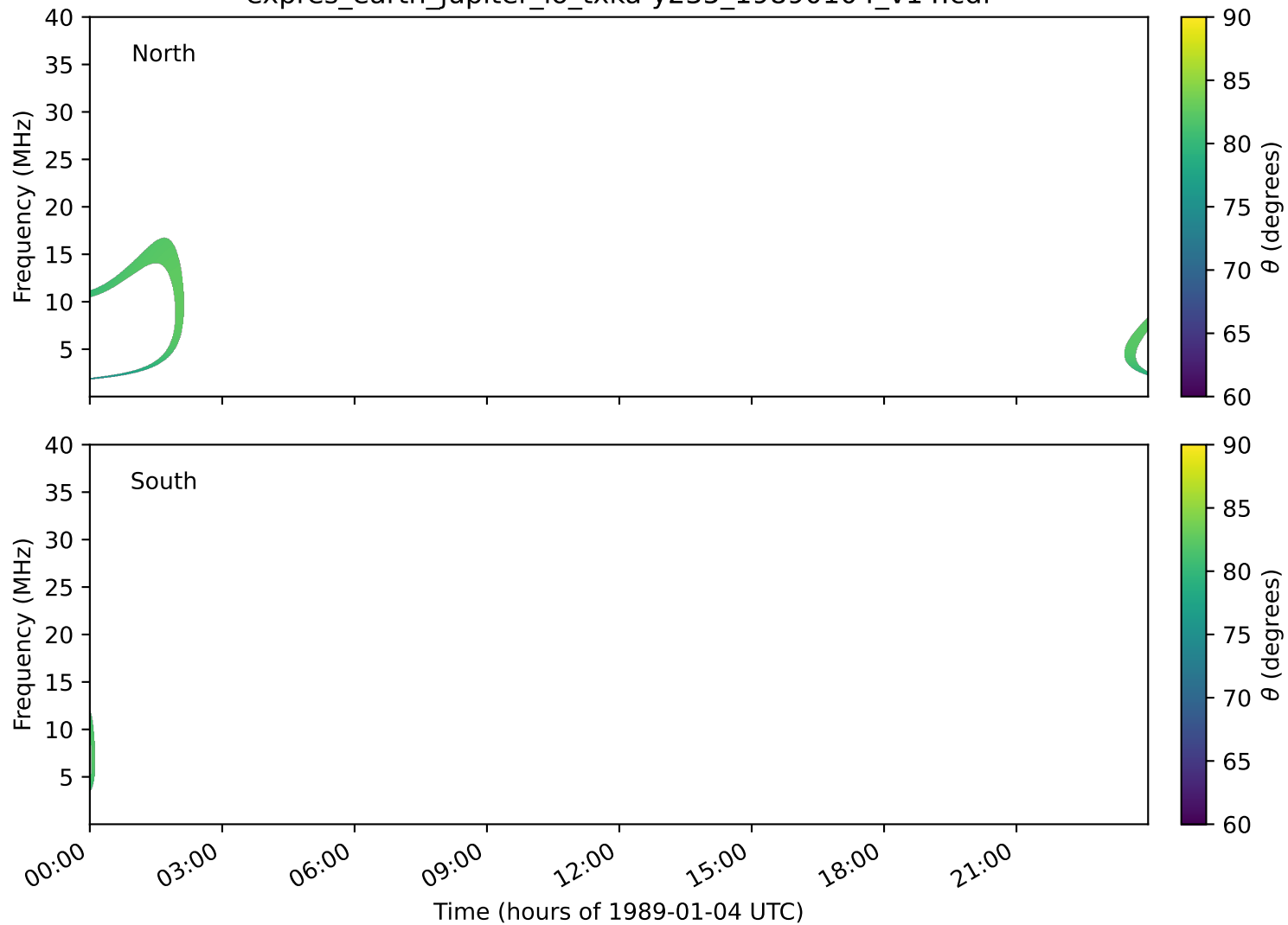
expres_earth_jupiter_io_txka-y235_19890104_v14.cdf
