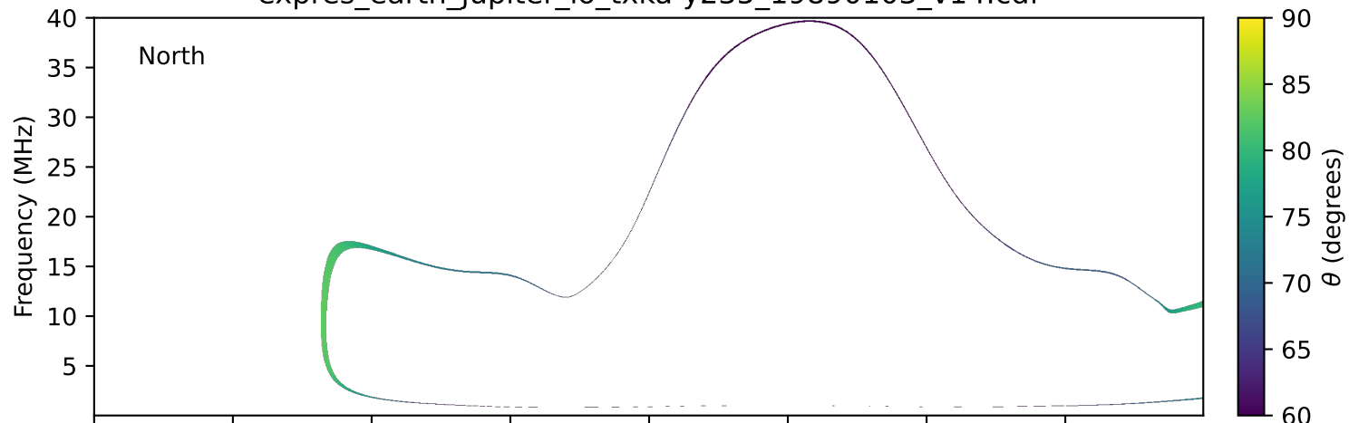
expres_earth_jupiter_io_txka-y235_19890103_v14.cdf
