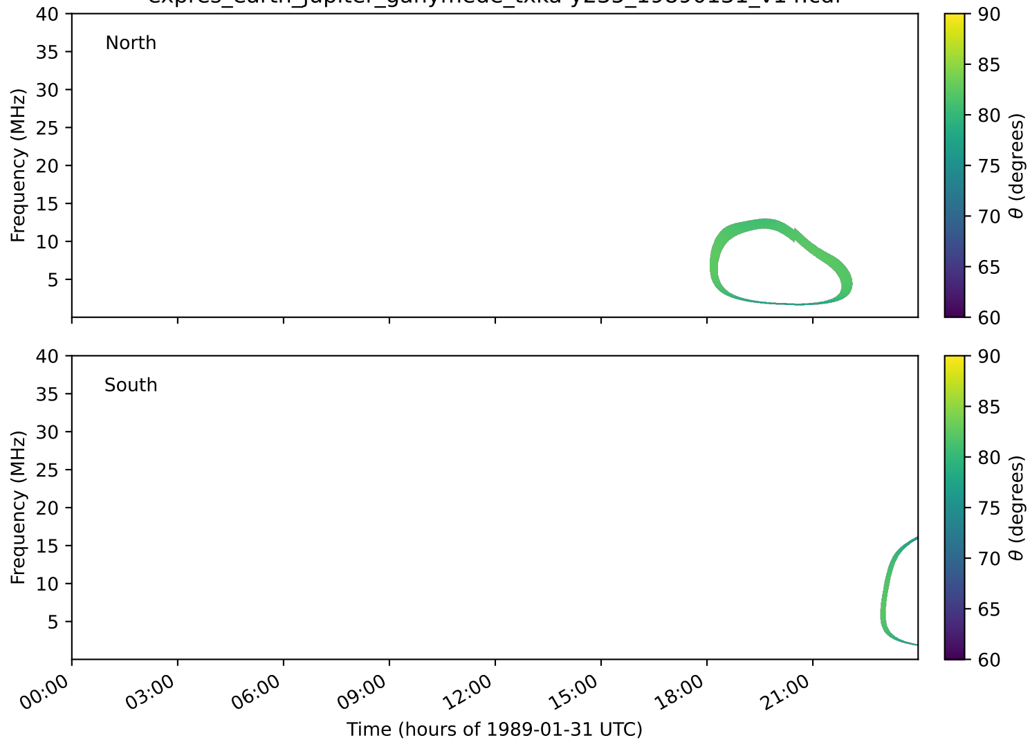
expres_earth_jupiter_ganymede_txka-y235_19890131_v14.cdf
