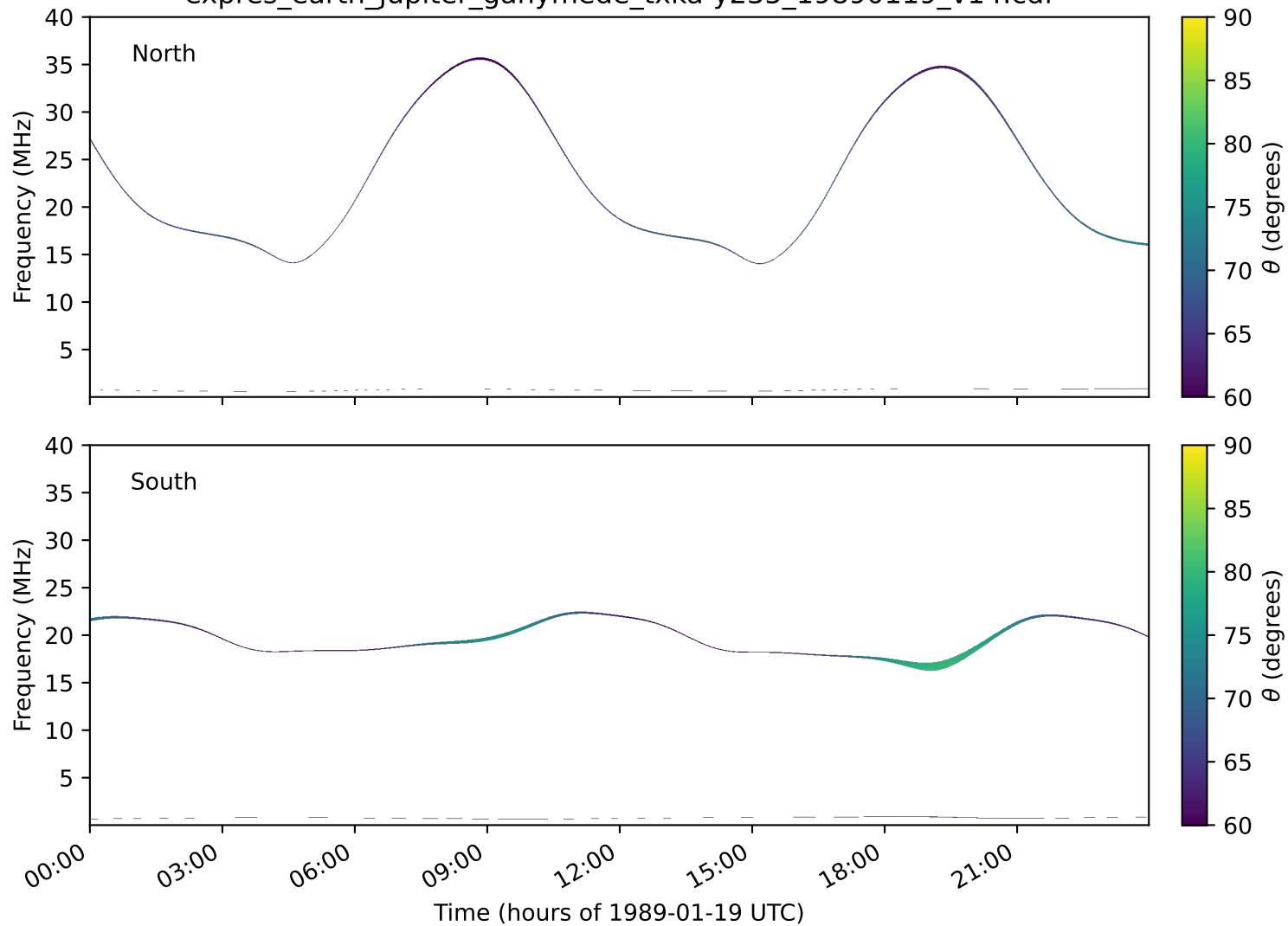
expres_earth_jupiter_ganymede_txka-y235_19890119_v14.cdf
