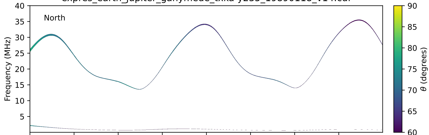
expres_earth_jupiter_ganymede_txka-y235_19890118_v14.cdf
