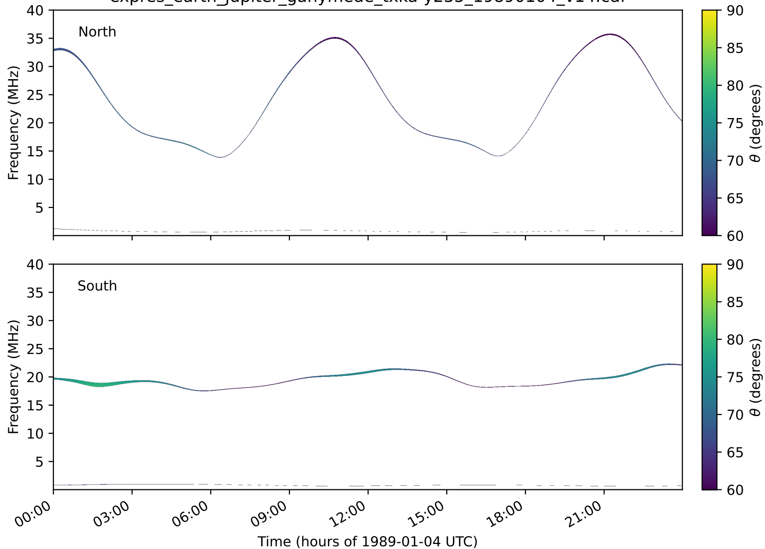
expres_earth_jupiter_ganymede_txka-y235_19890104_v14.cdf
