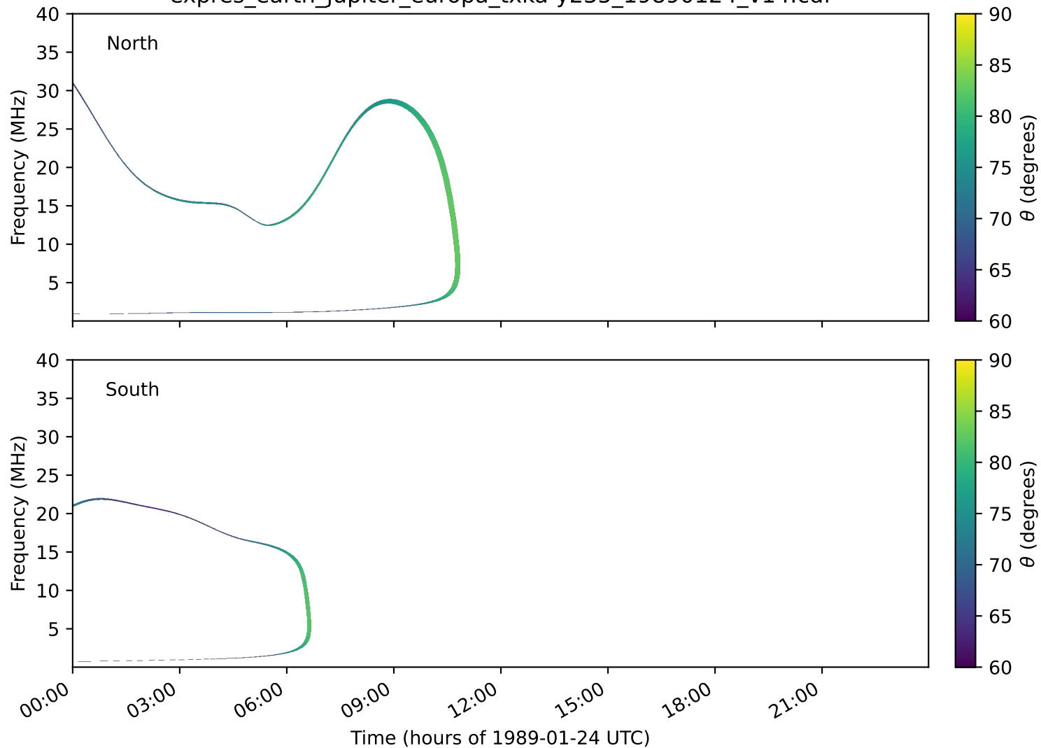
expres_earth_jupiter_europa_txka-y235_19890124_v14.cdf
