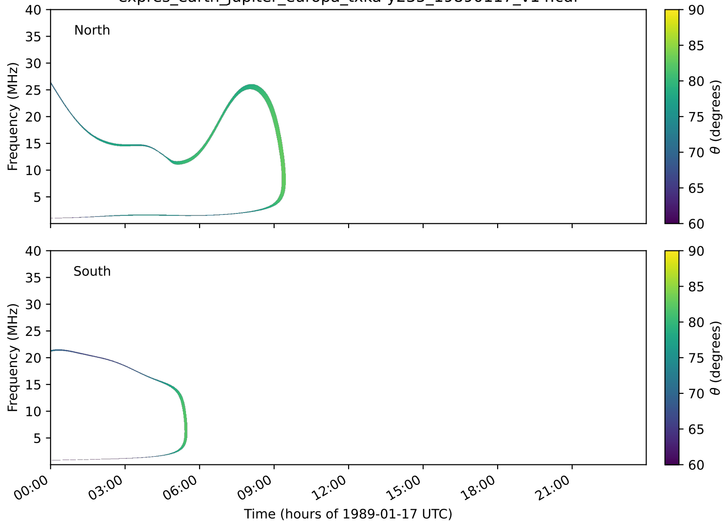
expres_earth_jupiter_europa_txka-y235_19890117_v14.cdf
