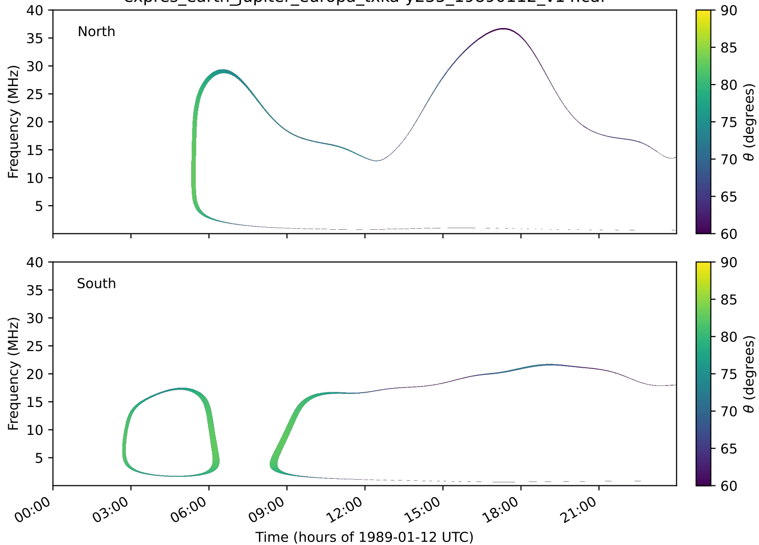
expres_earth_jupiter_europa_txka-y235_19890112_v14.cdf
