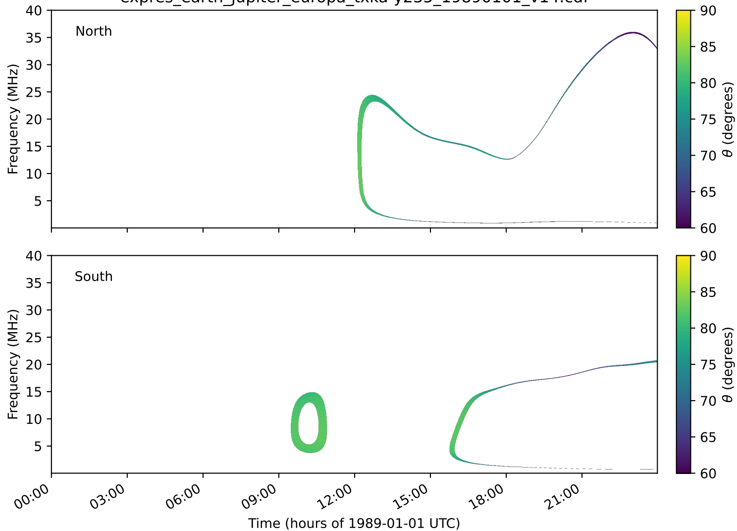
expres_earth_jupiter_europa_txka-y235_19890101_v14.cdf
