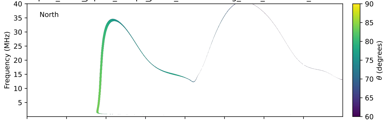
expres_earth_jupiter_europa_jrm09_lossc-wid1deg_3kev_19890112_v11.cdf
