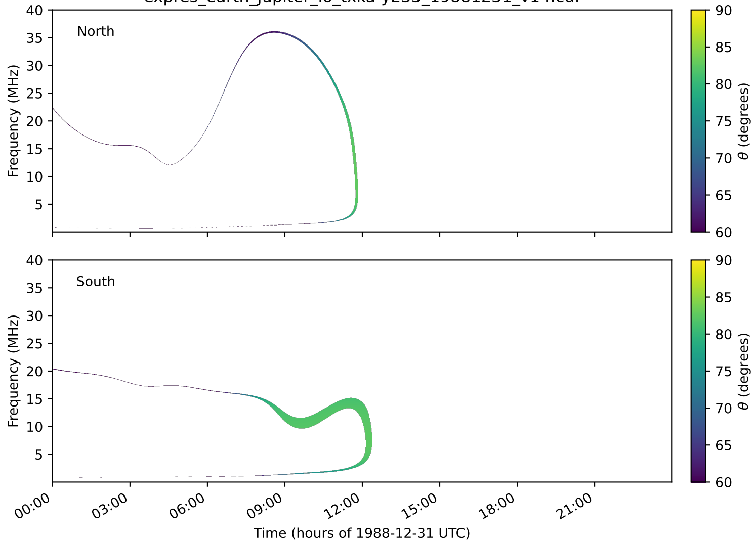
expres_earth_jupiter_io_txka-y235_19881231_v14.cdf
