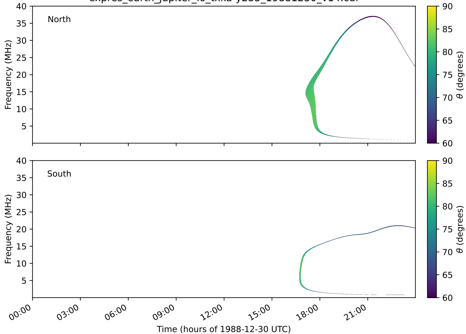
expres_earth_jupiter_io_txka-y235_19881230_v14.cdf
