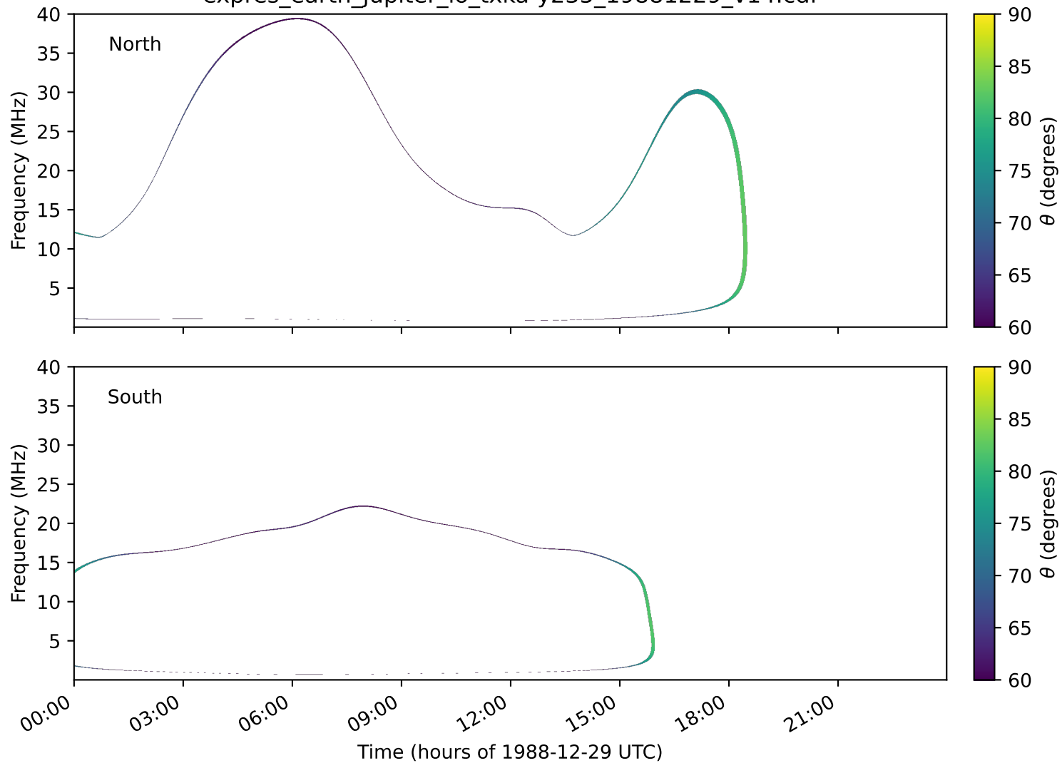
expres_earth_jupiter_io_txka-y235_19881229_v14.cdf
