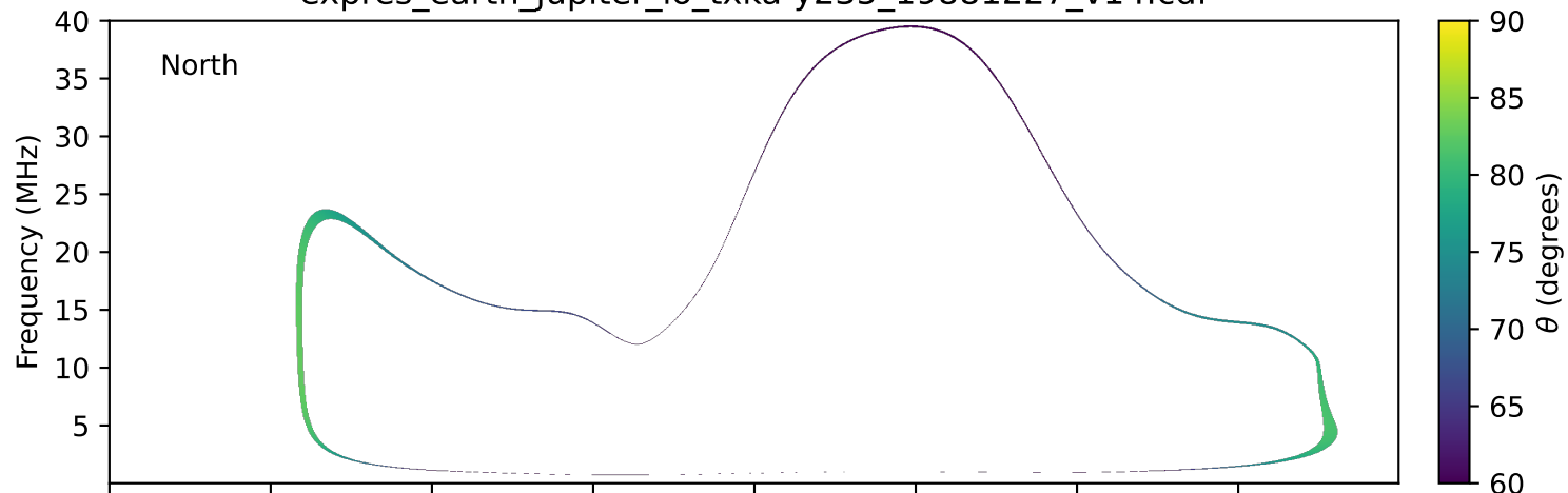
expres_earth_jupiter_io_txka-y235_19881227_v14.cdf
