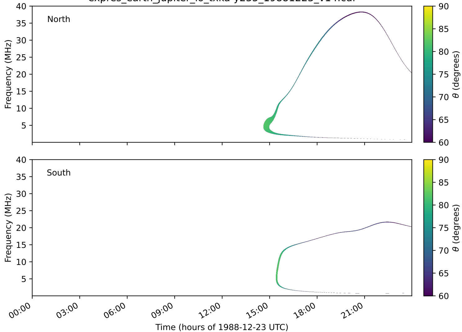
expres_earth_jupiter_io_txka-y235_19881223_v14.cdf
