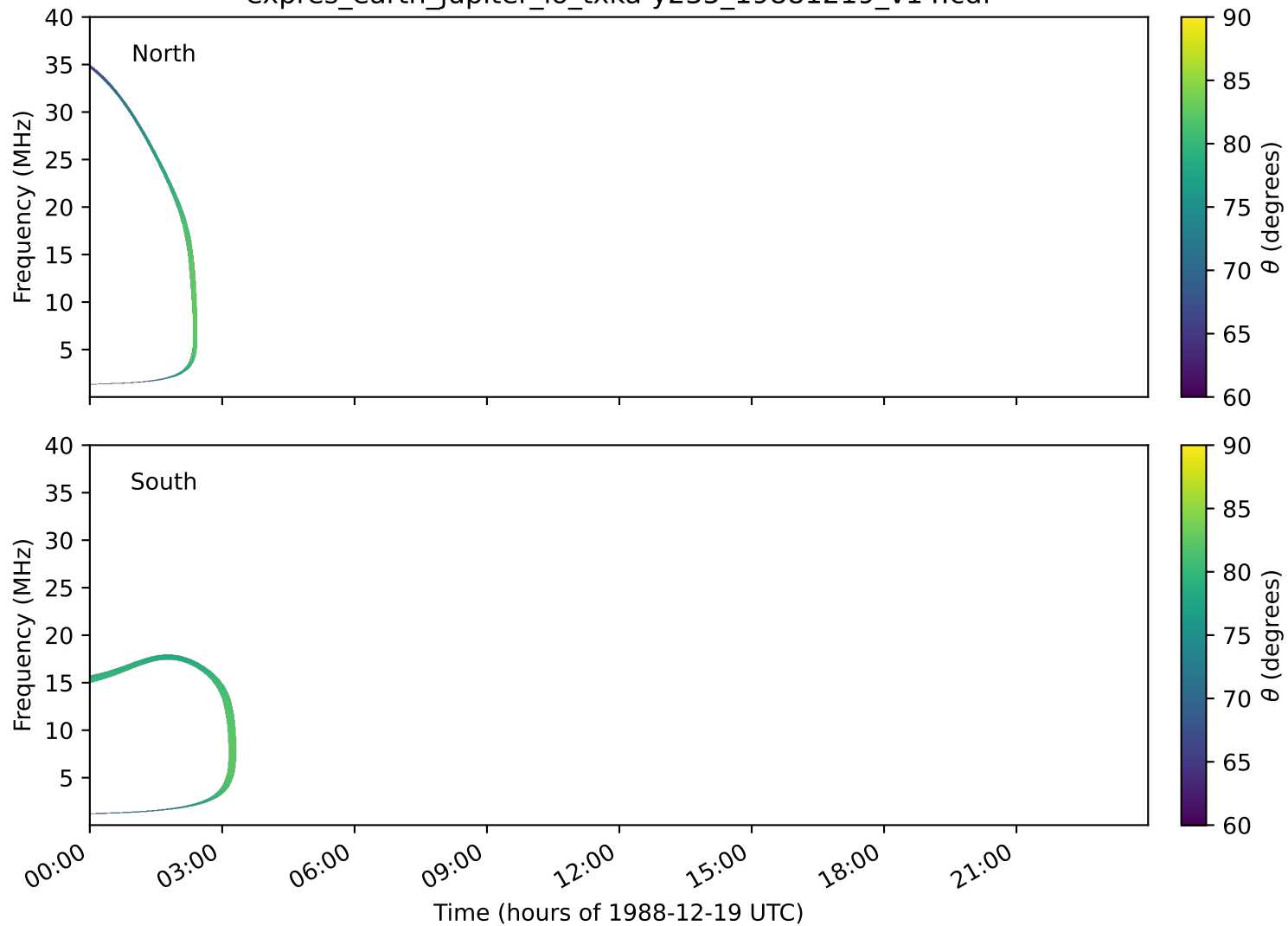
expres_earth_jupiter_io_txka-y235_19881219_v14.cdf
