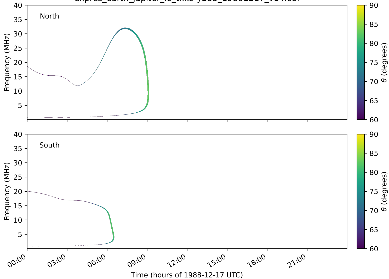
expres_earth_jupiter_io_txka-y235_19881217_v14.cdf
