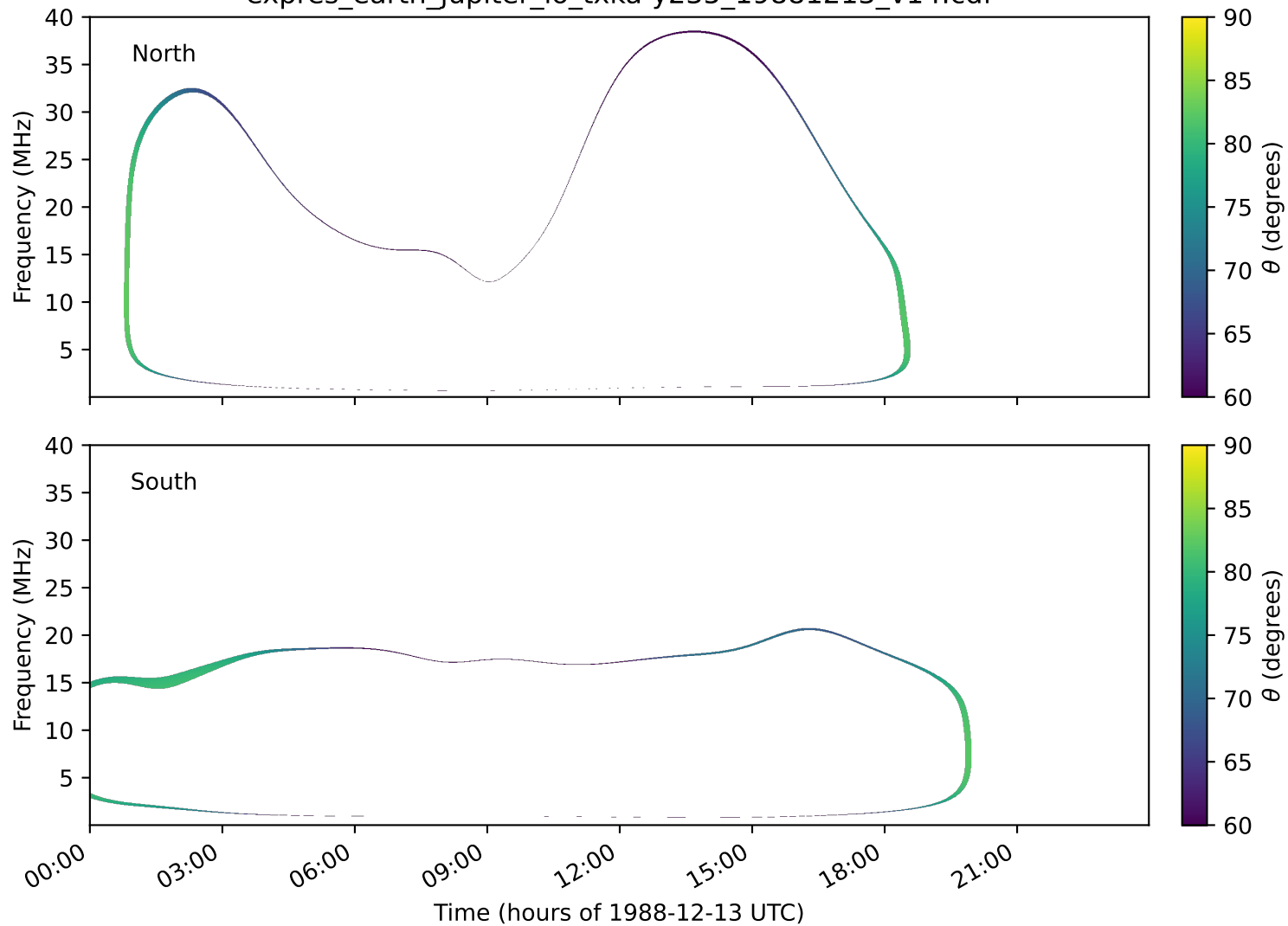
expres_earth_jupiter_io_txka-y235_19881213_v14.cdf
