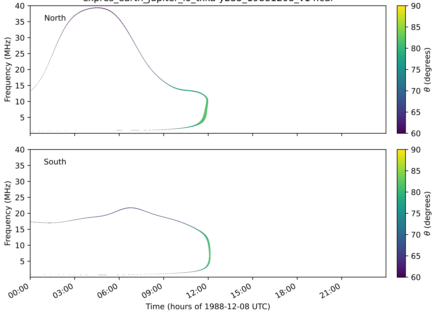
expres_earth_jupiter_io_txka-y235_19881208_v14.cdf
