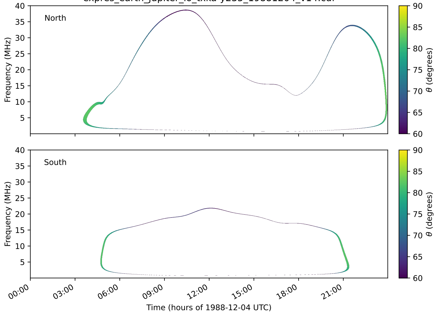
expres_earth_jupiter_io_txka-y235_19881204_v14.cdf
