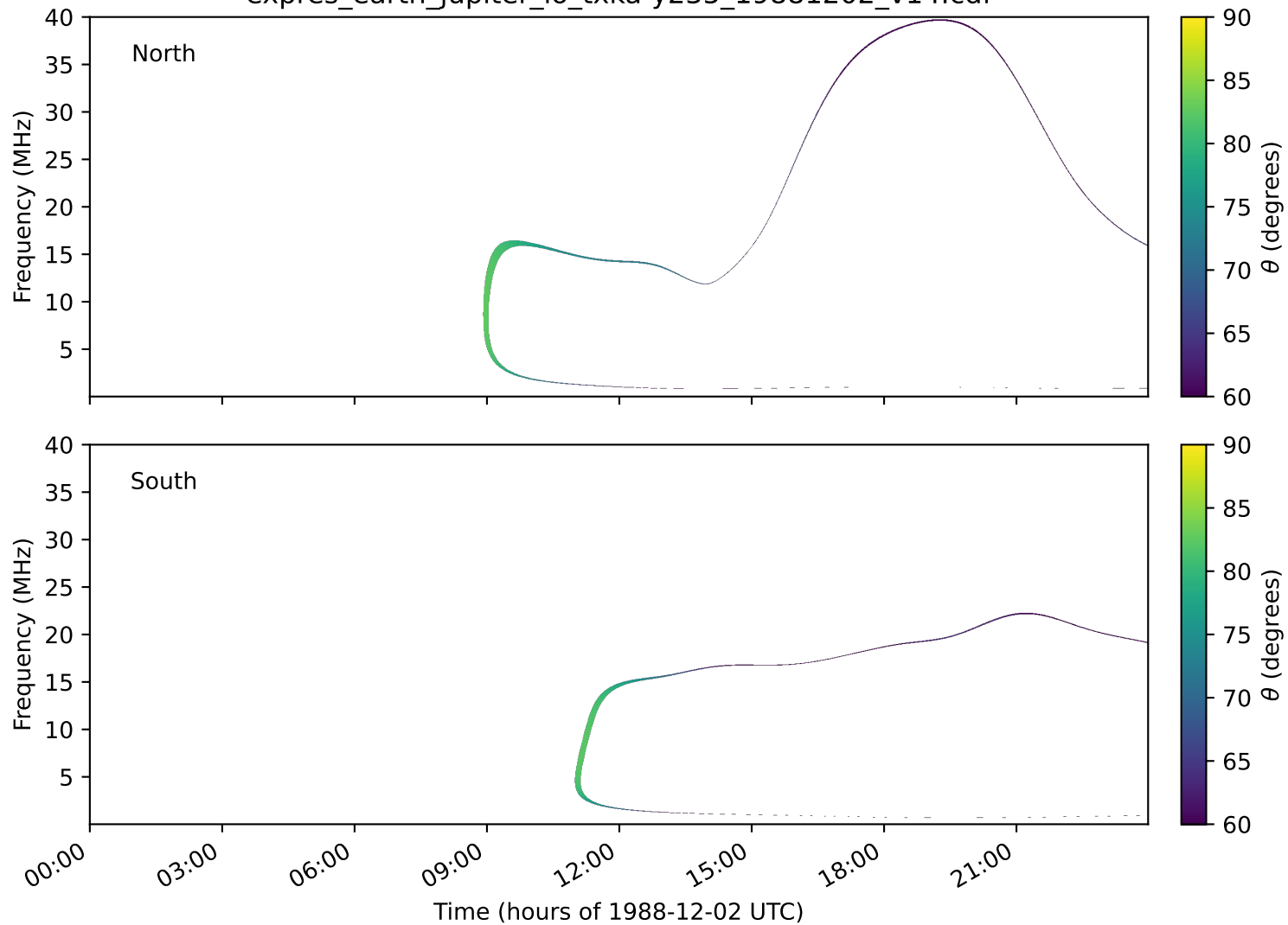
expres_earth_jupiter_io_txka-y235_19881202_v14.cdf
