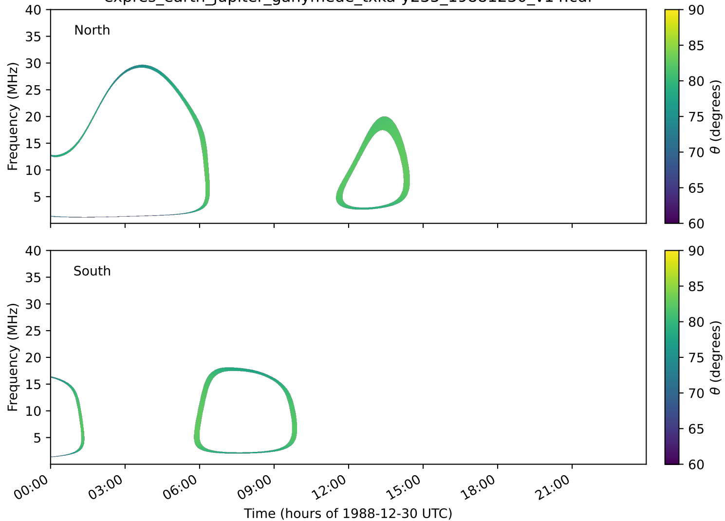
expres_earth_jupiter_ganymede_txka-y235_19881230_v14.cdf
