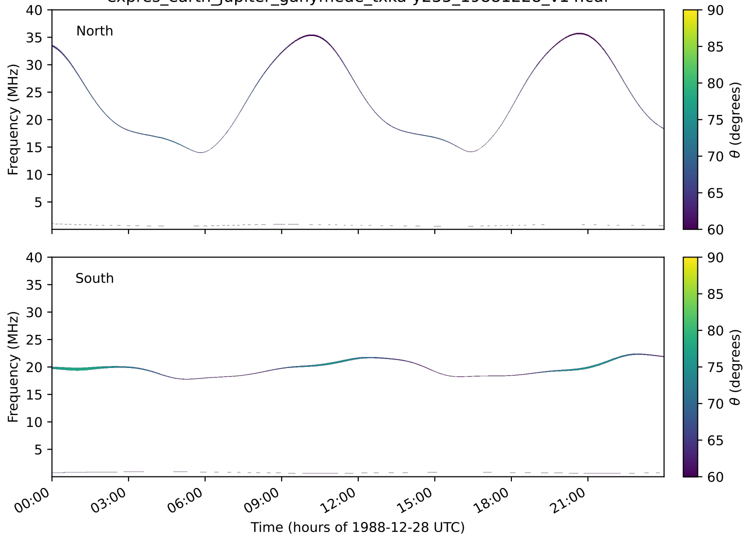
expres_earth_jupiter_ganymede_txka-y235_19881228_v14.cdf
