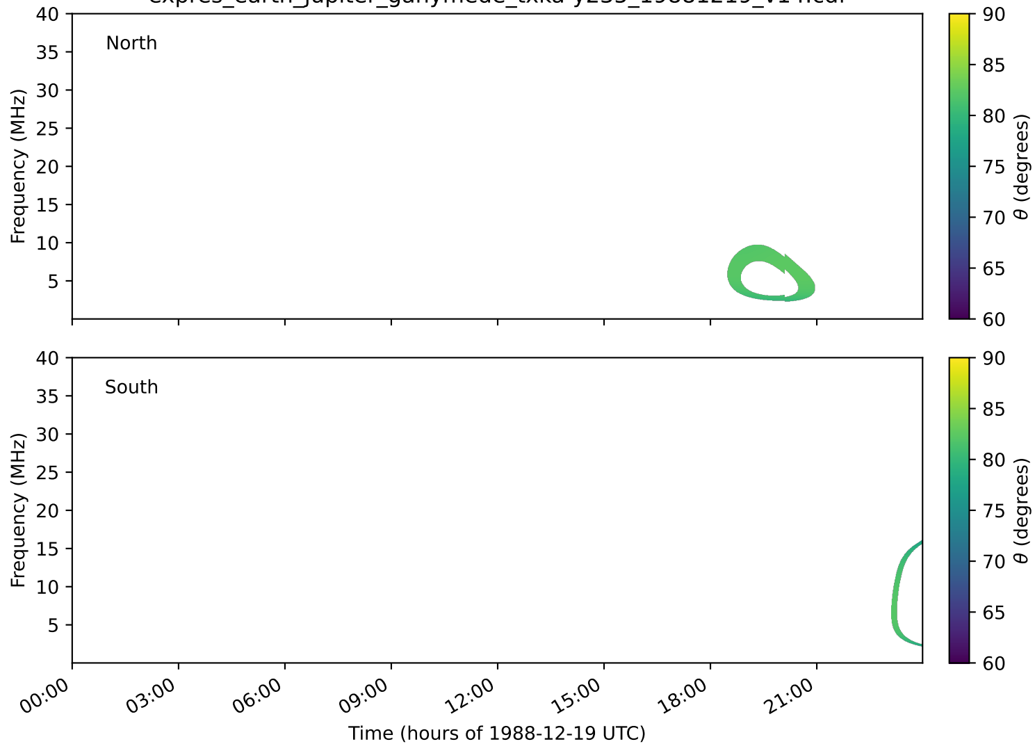
expres_earth_jupiter_ganymede_txka-y235_19881219_v14.cdf
