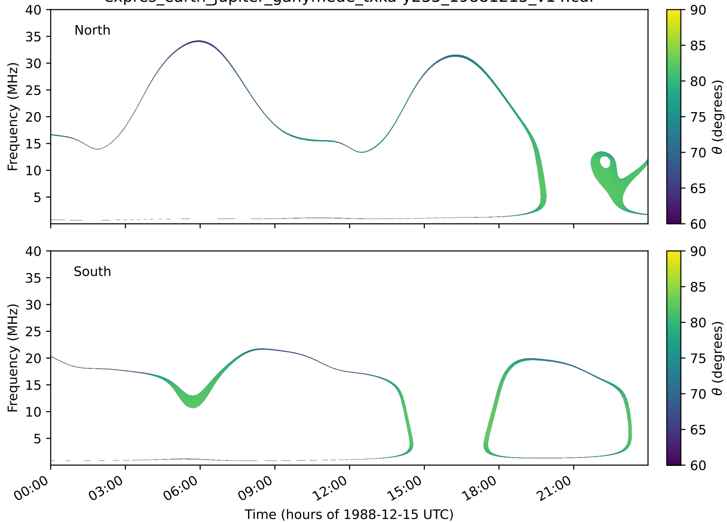
expres_earth_jupiter_ganymede_txka-y235_19881215_v14.cdf
