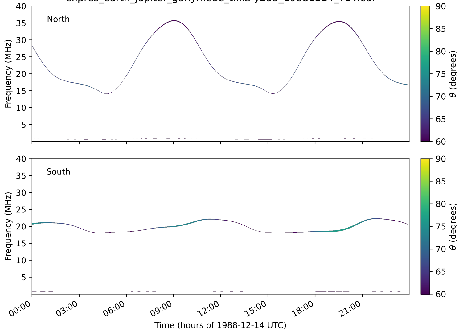
expres_earth_jupiter_ganymede_txka-y235_19881214_v14.cdf
