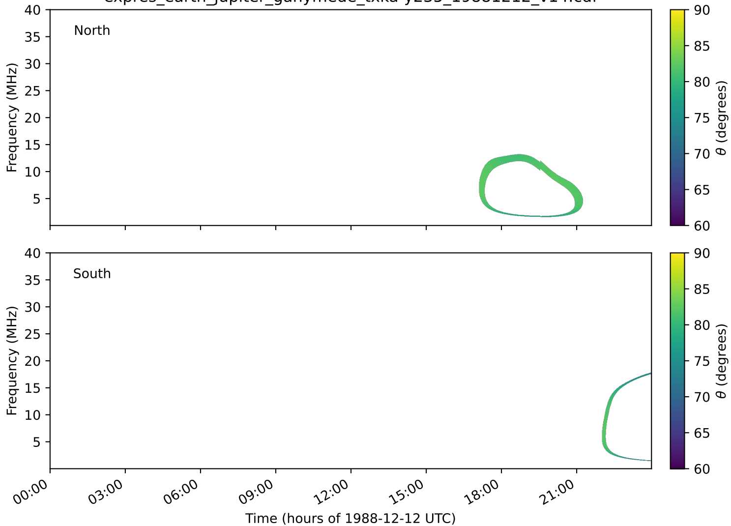
expres_earth_jupiter_ganymede_txka-y235_19881212_v14.cdf
