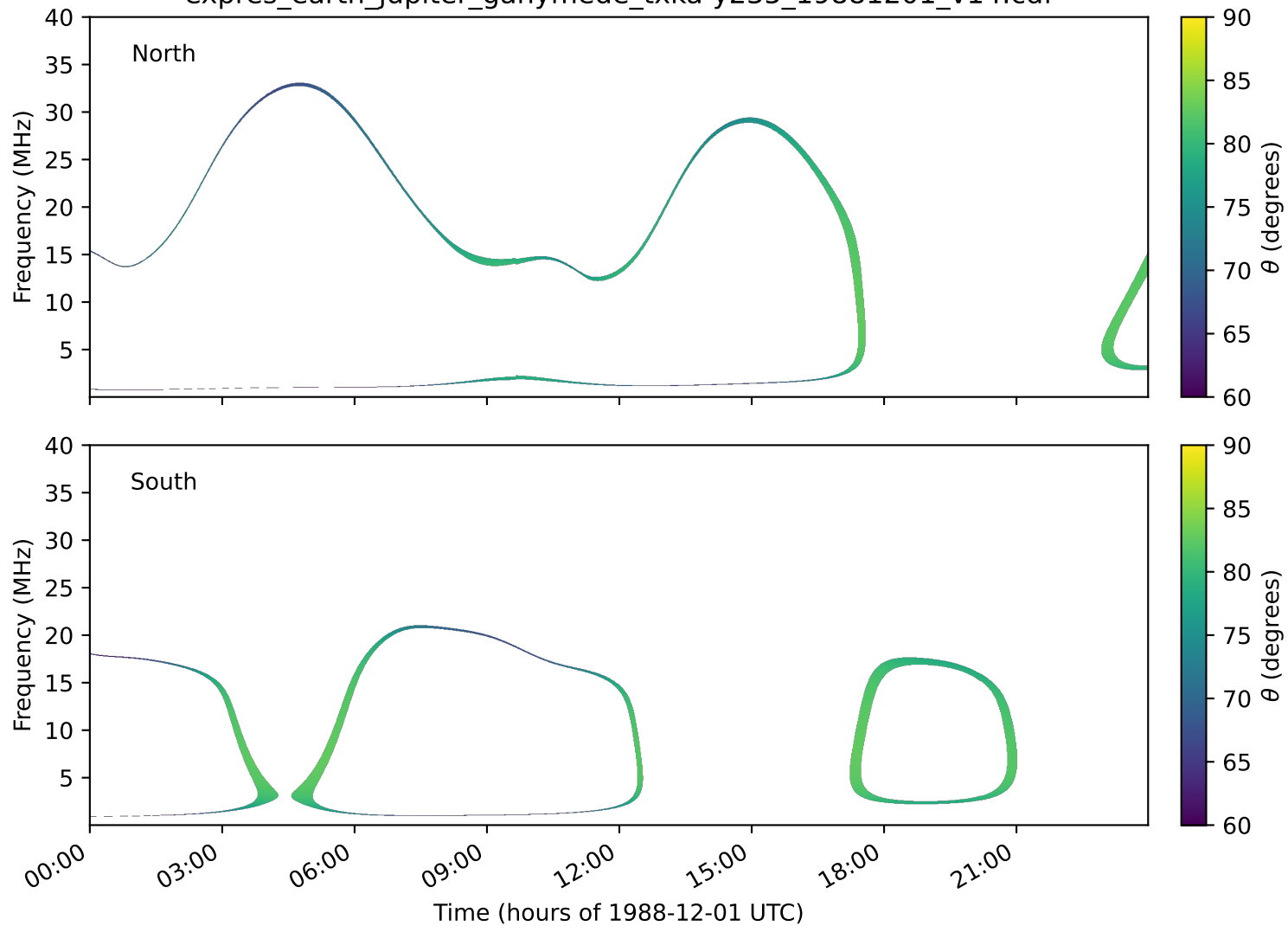
expres_earth_jupiter_ganymede_txka-y235_19881201_v14.cdf
