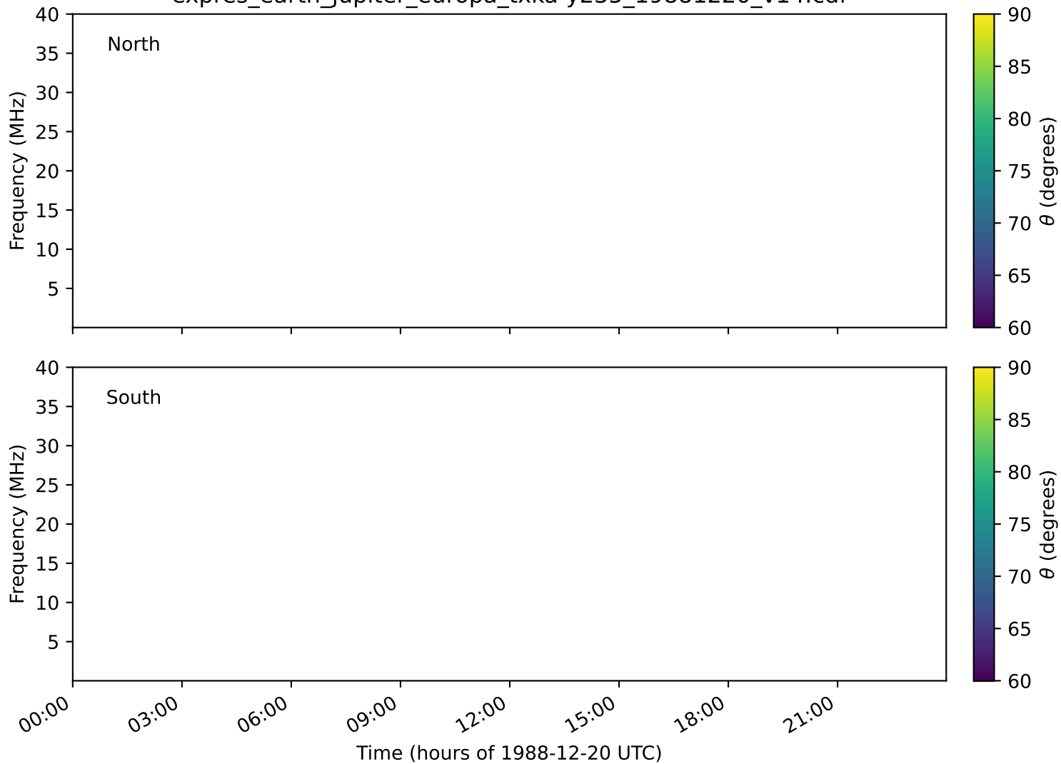
expres_earth_jupiter_europa_txka-y235_19881220_v14.cdf
